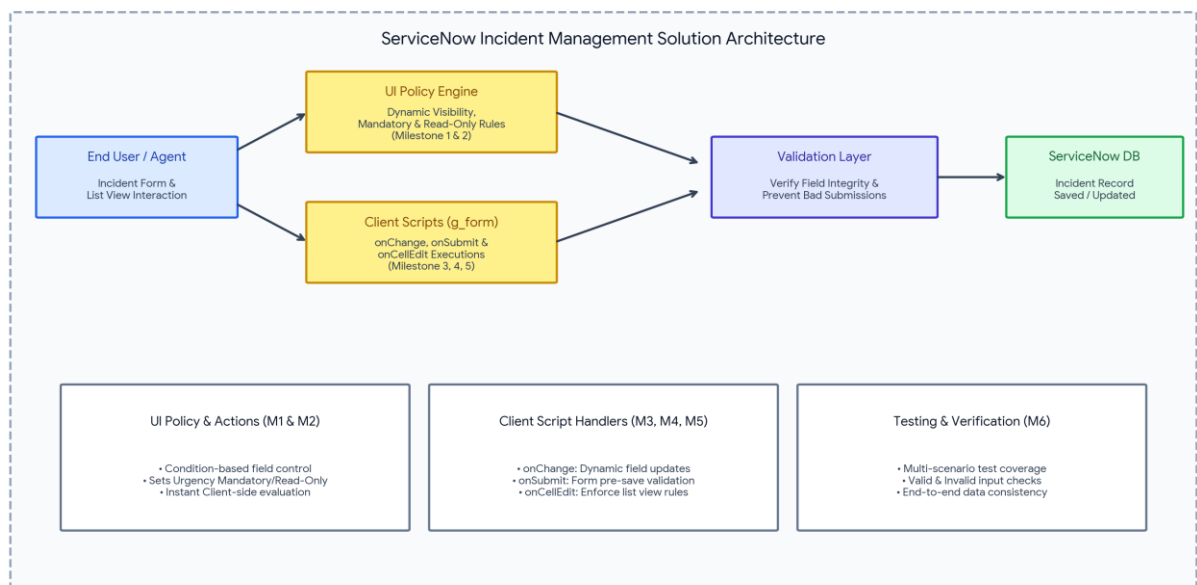
Figure 1: Architecture and data flow of the ServiceNow Incident Client Script & UI Policy solution
